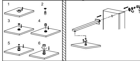
Head shower installation guide
