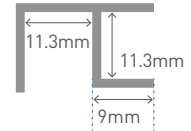
100. Flush Corner
